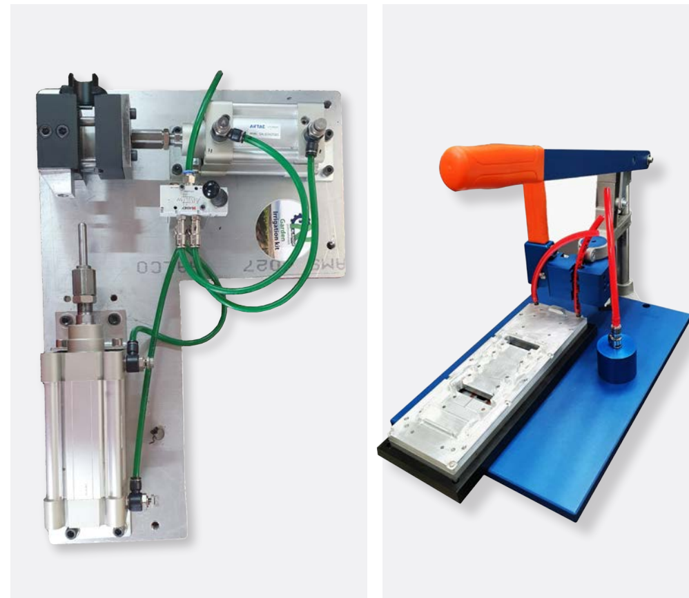
440507 Custom PI Manual Inserting Machine
