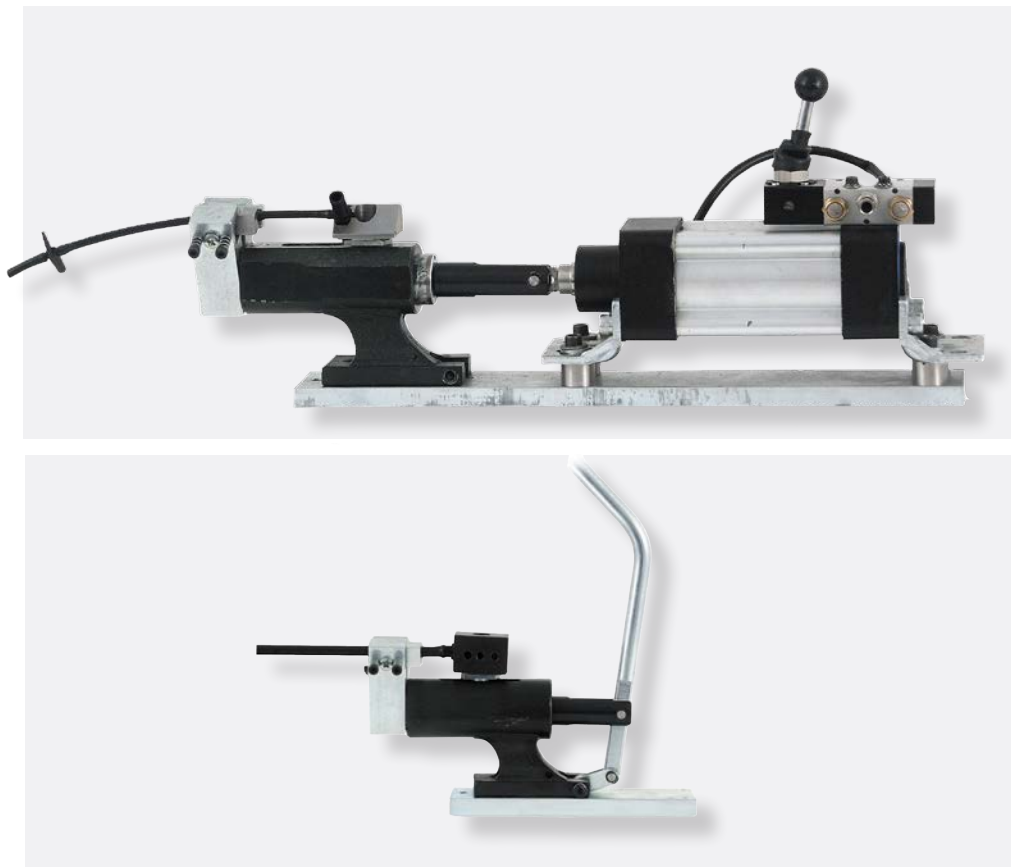
440501 MI Manual Inserting Machine
