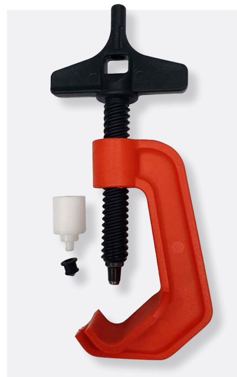
500006-P QDS-WDP-6mm – Punch& Inserter for woodpecker holes on pipe up to 32mm (including 10 seal cups)
