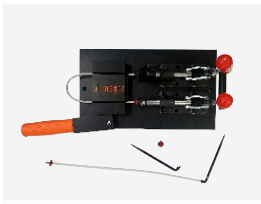
MI- Manual Inserting machine for NETAfim PCJ and Stick Arrow dripper
