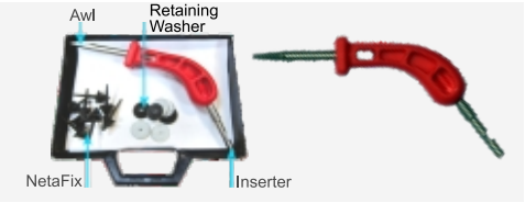
801777 NETAFIX tool for repairing holes in LAYFLAT hose with Netafim sealing caps.
